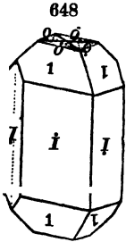
Strontian.
